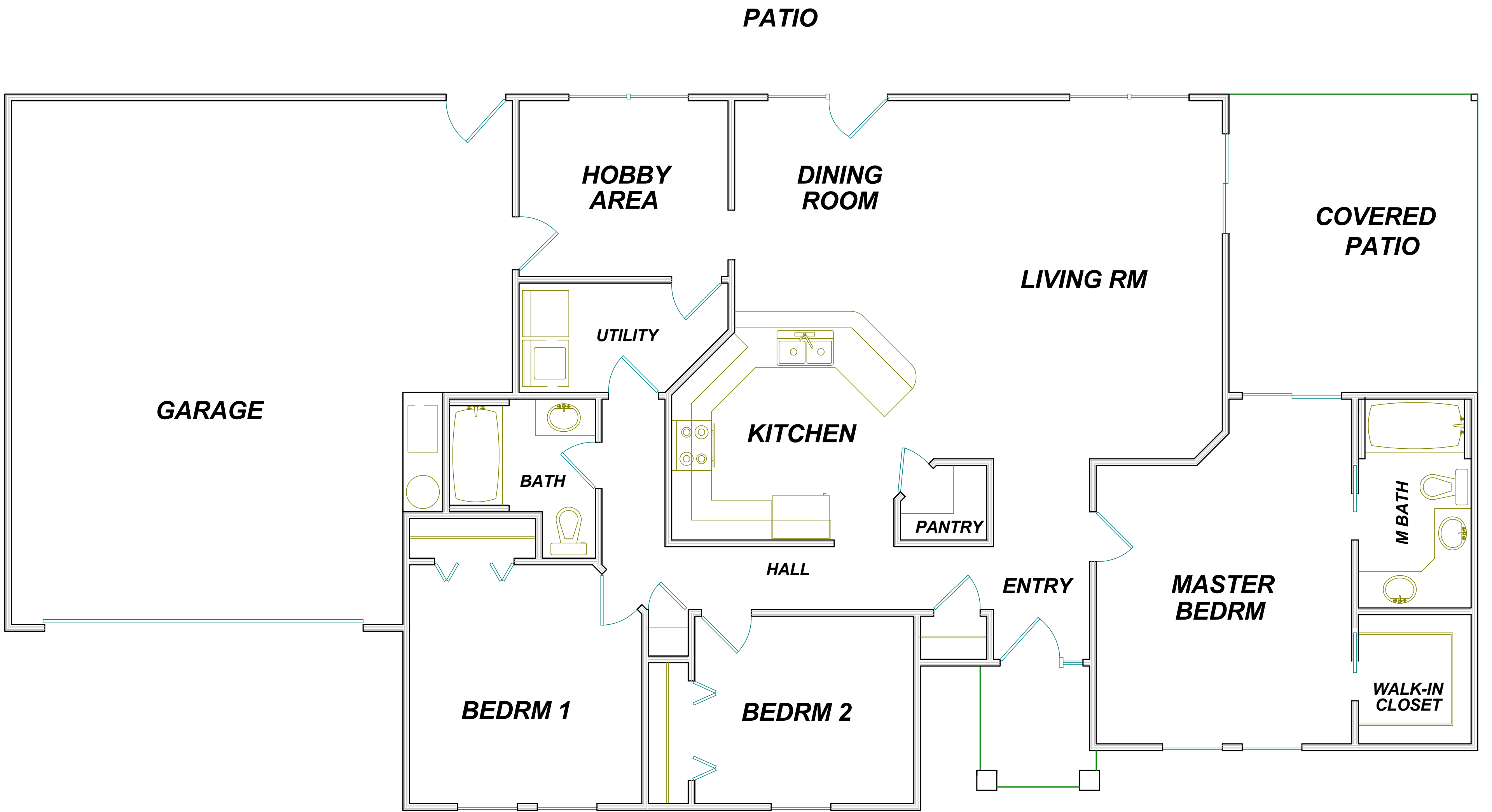
1540 SQ FT DWELLING
